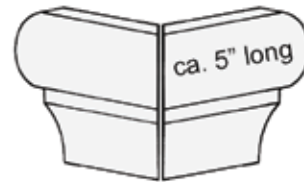
V1.5xCap mitered Cmr (2 pieces - 1.5"x 5" ea.)
